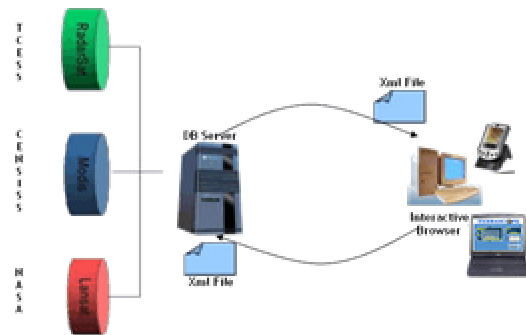
Figure 1. Terrascope Architecture
