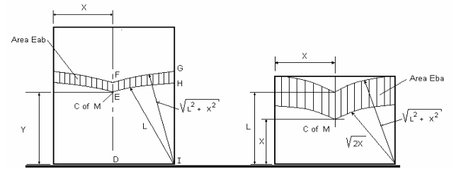
Figure1. Energy barrier for a squared prism [1].
